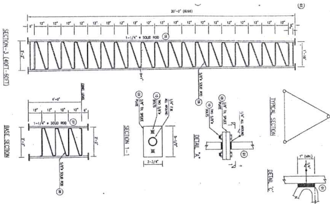
Figure 11: Schematic 3-Tower
