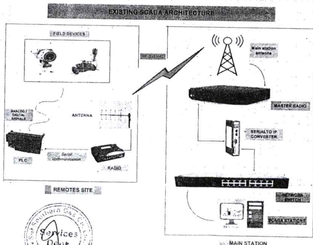
Figure 2: SCADA Architecture
