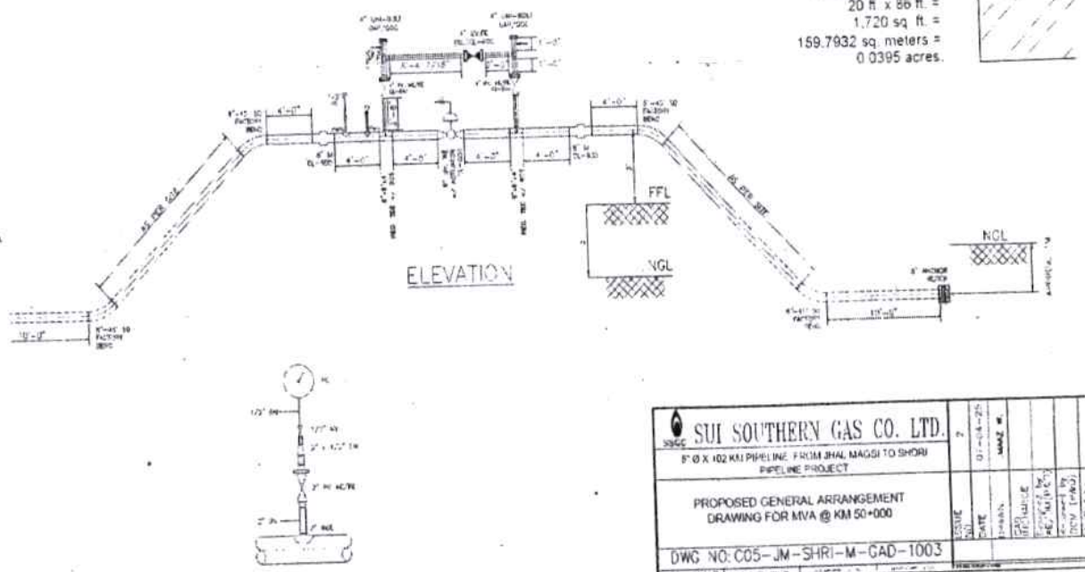
Figure 5: Schematic MVA-50
