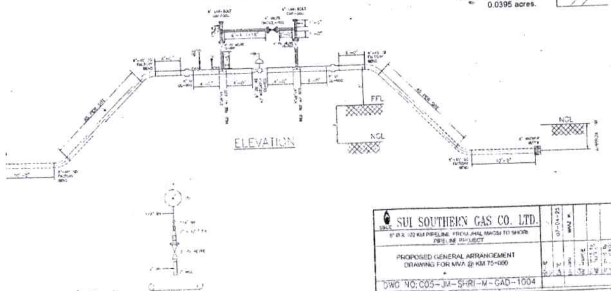
Figure 6: Schematic MVA-75
