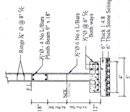
TYPICAL COLUMN FOUNDATION
