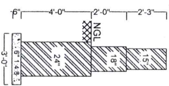
WALL SECTION - AA
