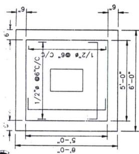
PLAN OF RCC COLUMN FOUNDATION (TYP)
