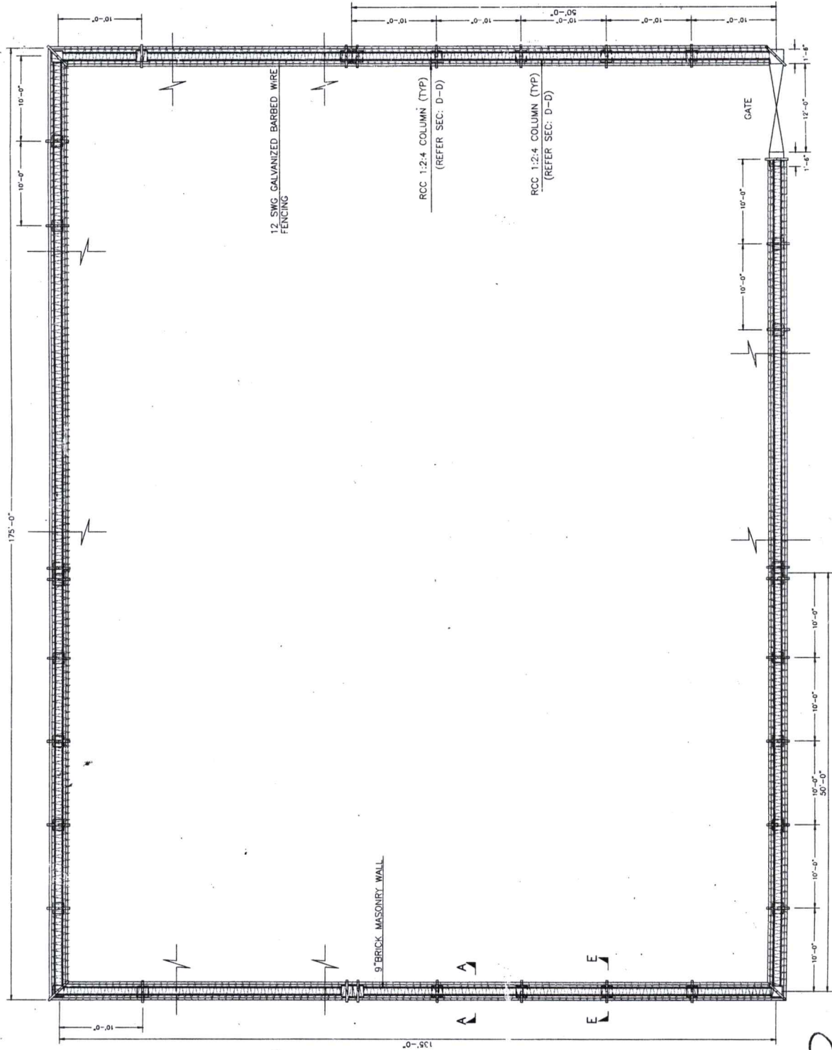
PROPOSED BOUNDARY WALL ENCLOSURE PLAN FOR
