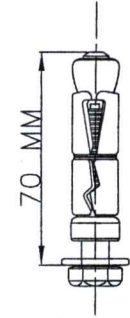
M10 RAWAL BOLT DETAIL
